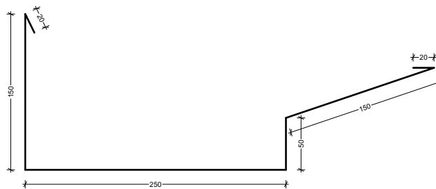
Box Gutter Detail SCALE NTS
